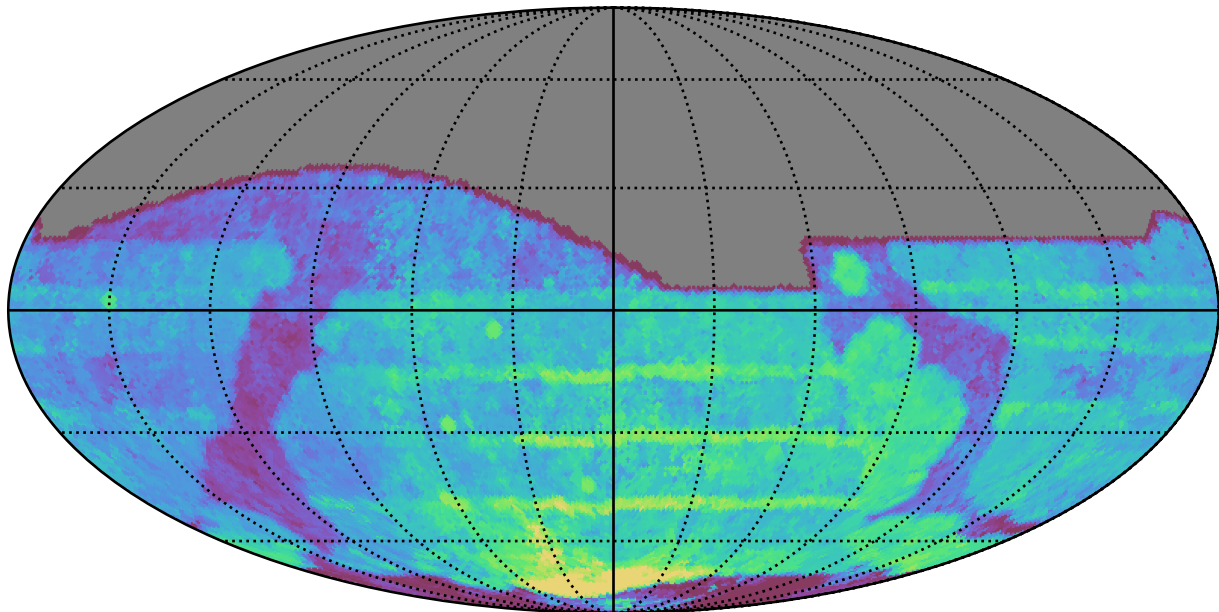
smc_lmc_v3.3_10yrs All sky all bands: Median Season Length
