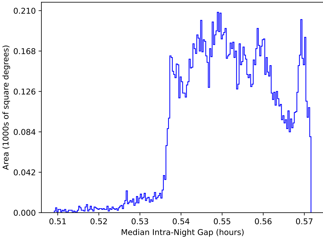
smc_lmc_v3.3_10yrs WFD: Median Intra-Night Gap
