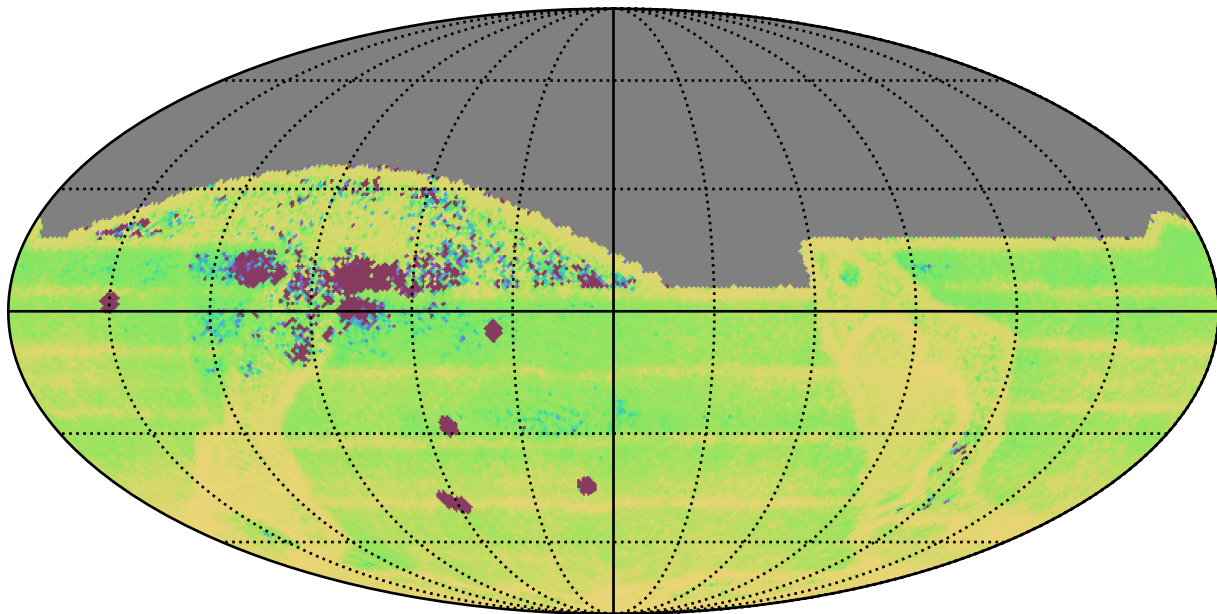
smc_lmc_v3.3_10yrs All sky: Median Intra-Night Gap
