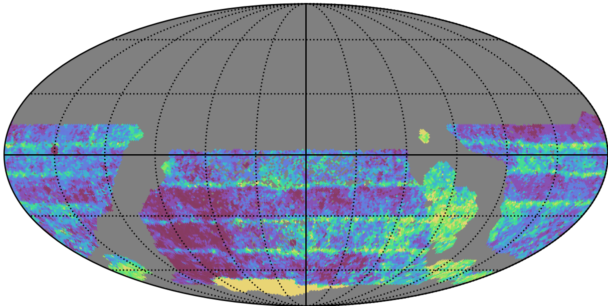
smc_lmc_v3.3_10yrs WFD z band: Median Inter-Night Gap
