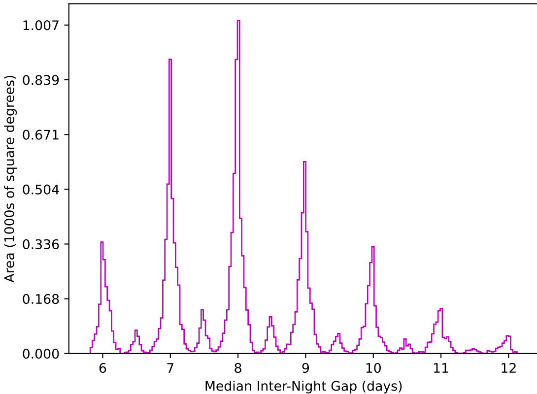
smc_lmc_v3.3_10yrs WFD z band: Median Inter-Night Gap
