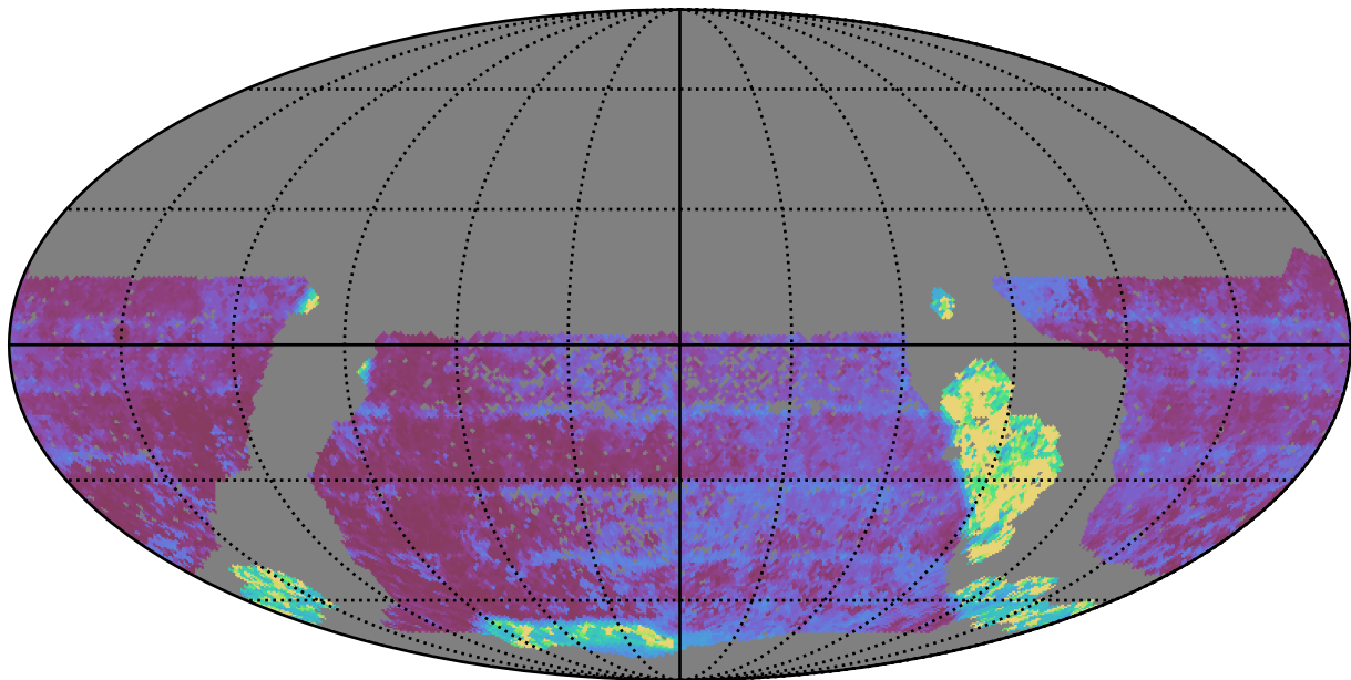
smc_lmc_v3.3_10yrs WFD y band: Median Inter-Night Gap
