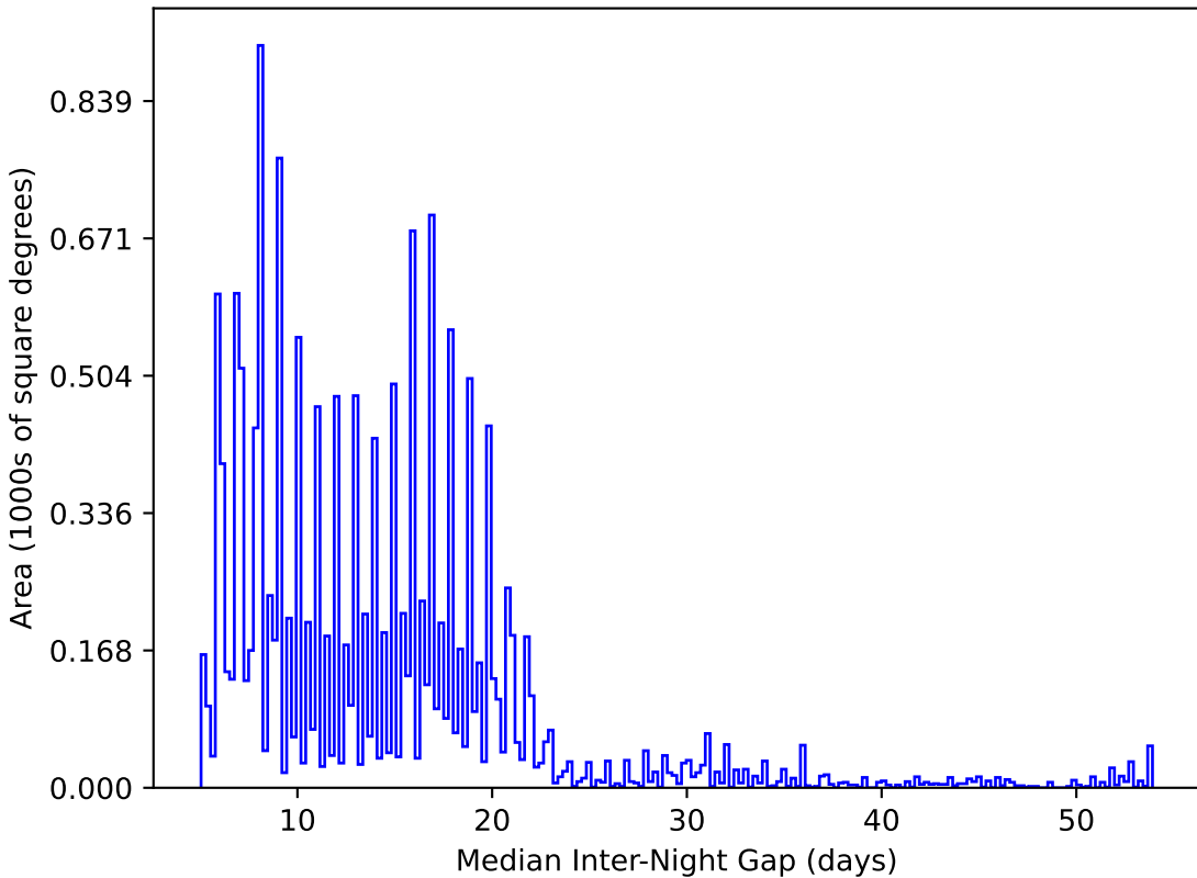
smc_lmc_v3.3_10yrs WFD y band: Median Inter-Night Gap
