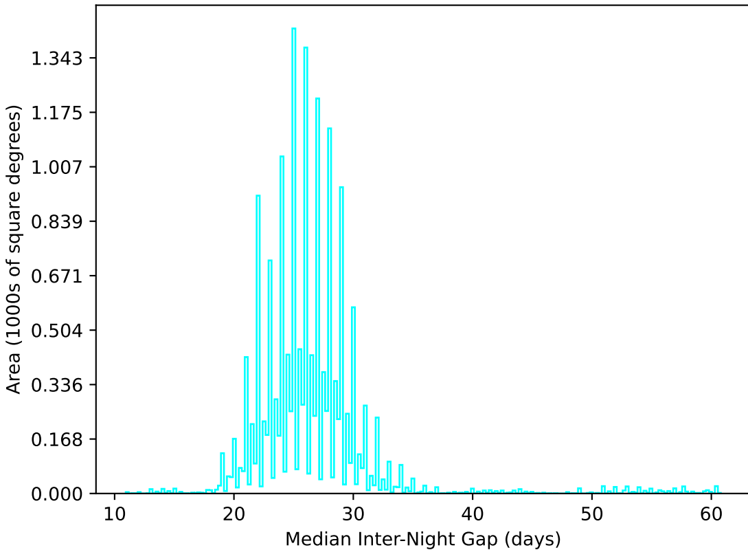
smc_lmc_v3.3_10yrs WFD u band: Median Inter-Night Gap
