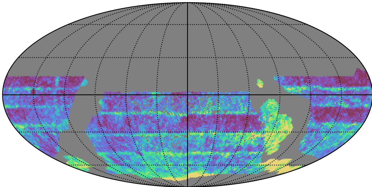
smc_lmc_v3.3_10yrs WFD r band: Median Inter-Night Gap
