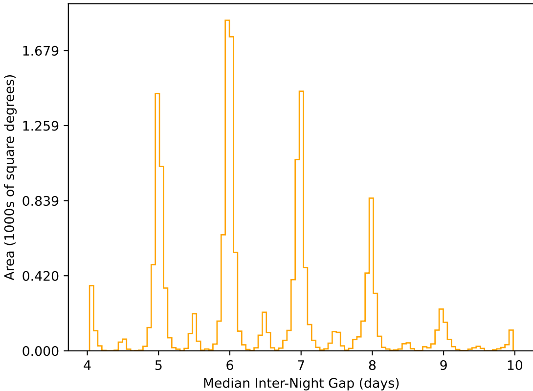
smc_lmc_v3.3_10yrs WFD r band: Median Inter-Night Gap
