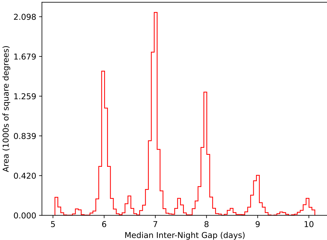
smc_lmc_v3.3_10yrs WFD i band: Median Inter-Night Gap
