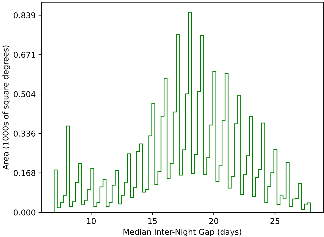
smc_lmc_v3.3_10yrs WFD g band: Median Inter-Night Gap
