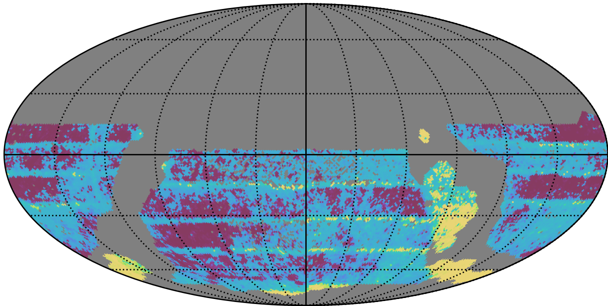
smc_lmc_v3.3_10yrs WFD all bands: Median Inter-Night Gap
