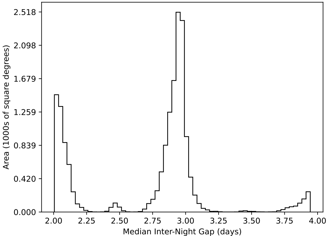
smc_Imc_v3.3_10yrs WFD all bands: Median Inter-Night Gap
