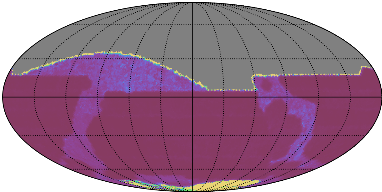
smc_lmc_v3.3_10yrs All sky z band: Median Inter-Night Gap
