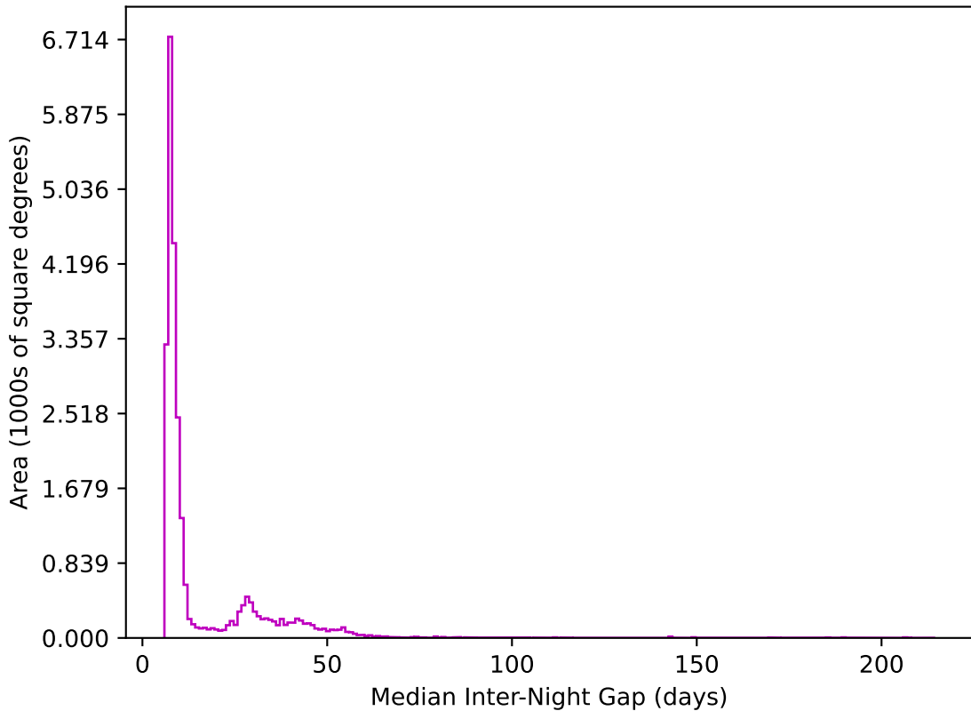
smc_lmc_v3.3_10yrs All sky z band: Median Inter-Night Gap
