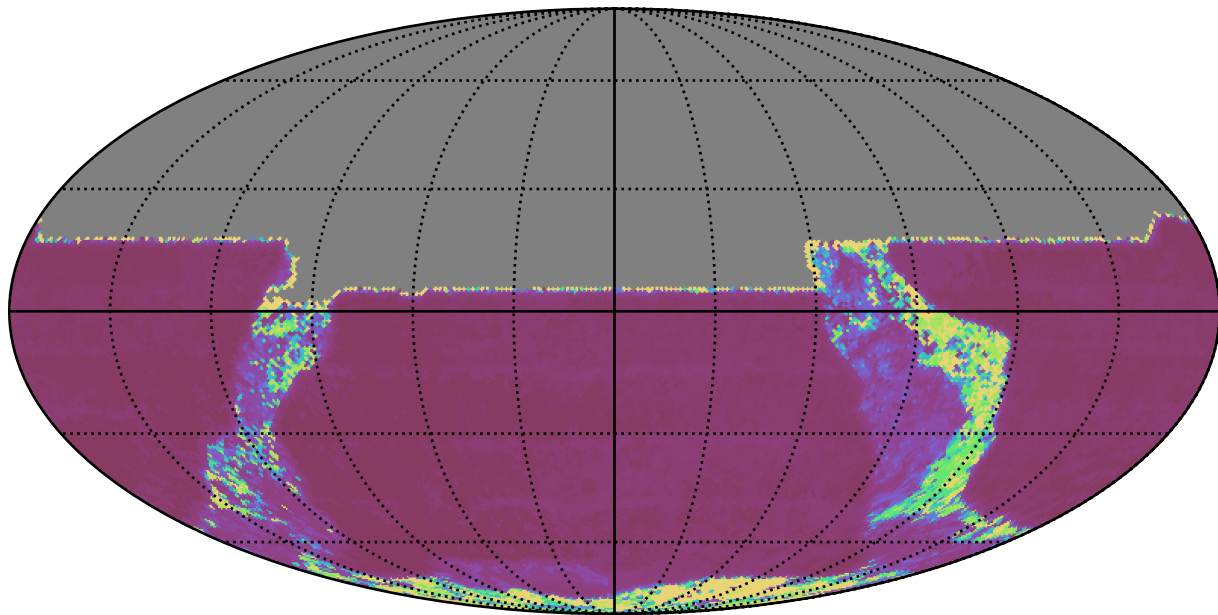
smc_lmc_v3.3_10yrs All sky y band: Median Inter-Night Gap
