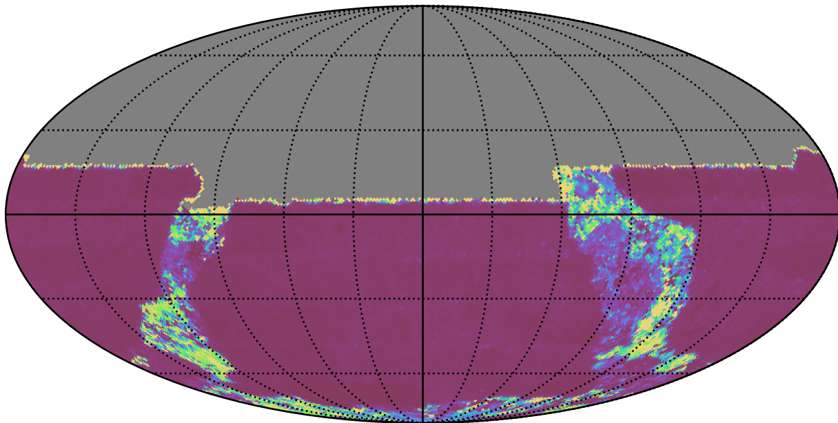
smc_lmc_v3.3_10yrs All sky u band: Median Inter-Night Gap
