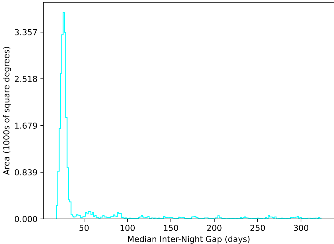
smc_lmc_v3.3_10yrs All sky u band: Median Inter-Night Gap
