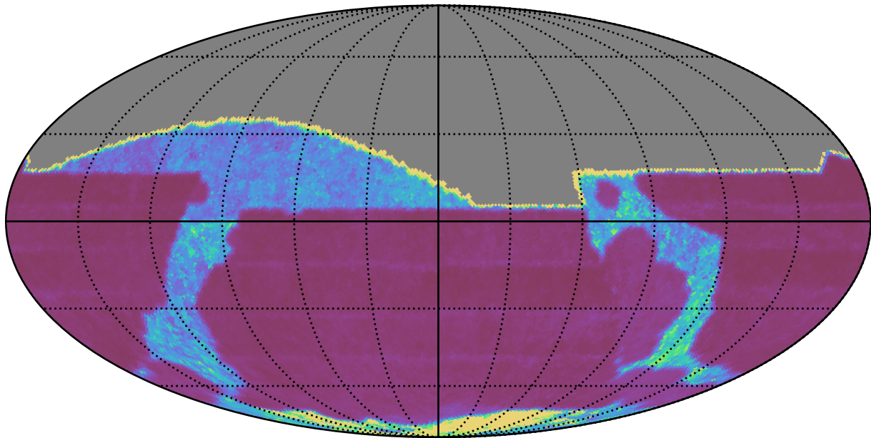
smc_lmc_v3.3_10yrs All sky r band: Median Inter-Night Gap
