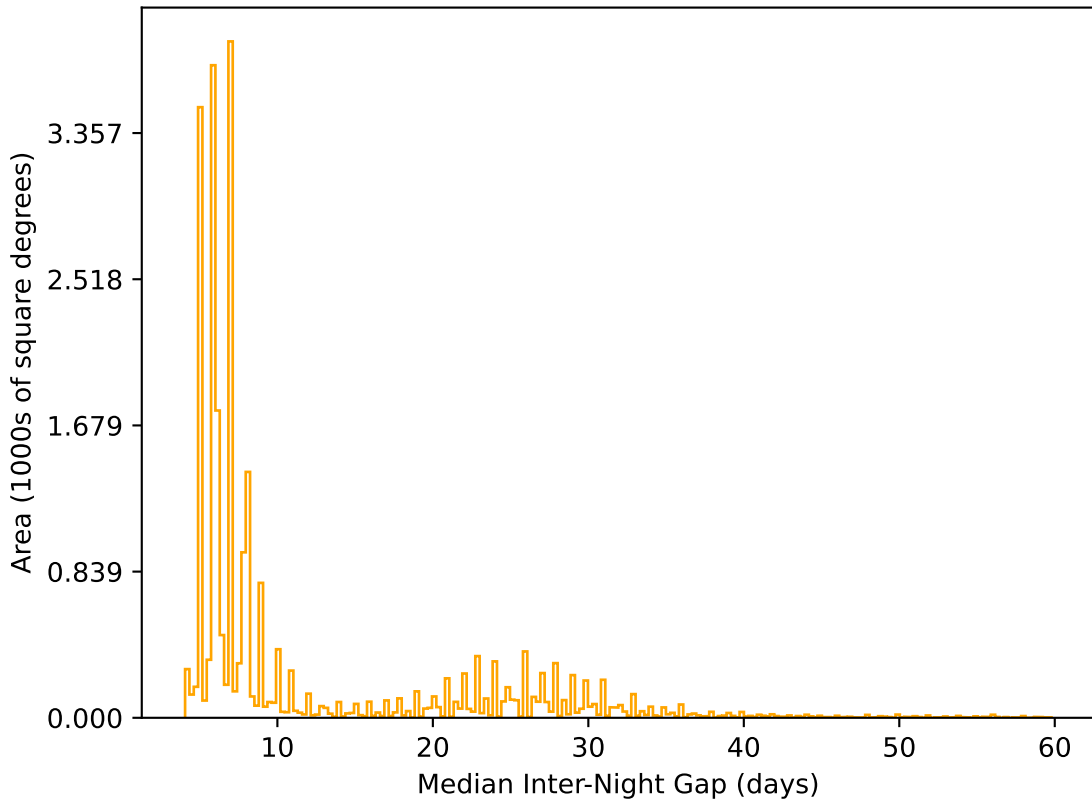
smc_lmc_v3.3_10yrs All sky r band: Median Inter-Night Gap
