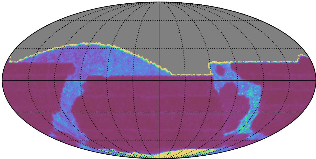
smc_lmc_v3.3_10yrs All sky i band: Median Inter-Night Gap
