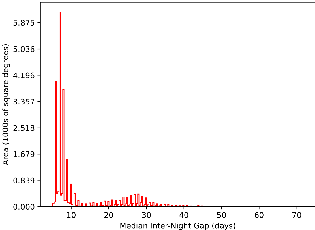
smc_lmc_v3.3_10yrs All sky i band: Median Inter-Night Gap
