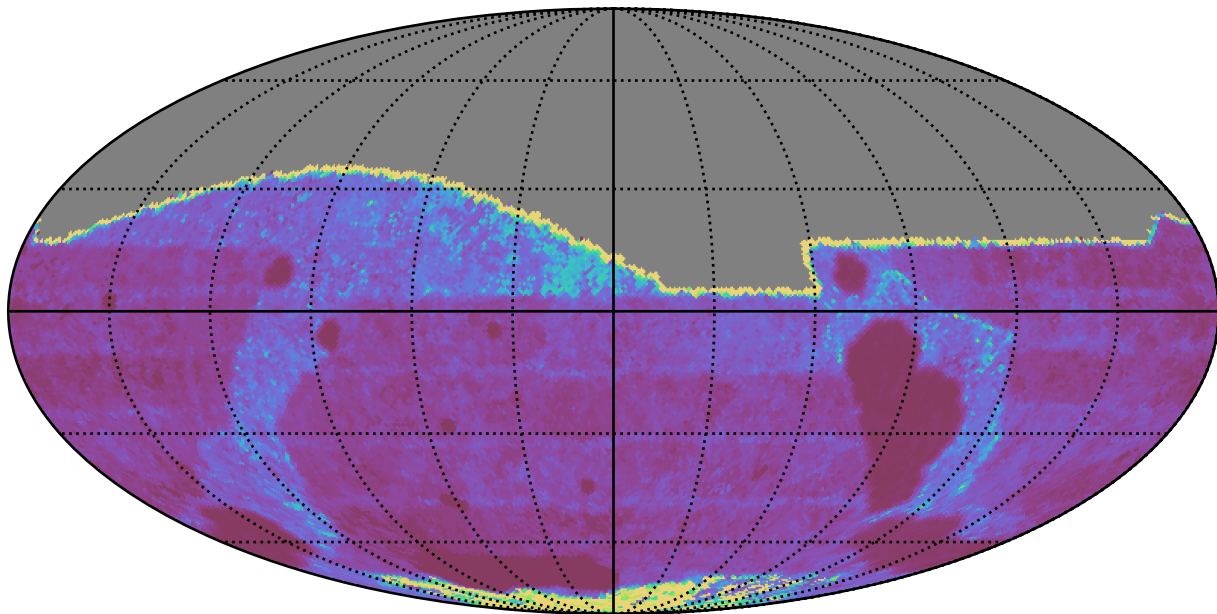
smc_lmc_v3.3_10yrs All sky g band: Median Inter-Night Gap
