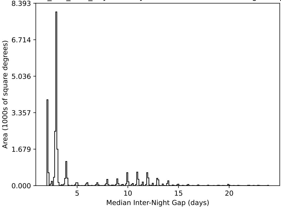
smc_lmc_v3.3_10yrs All sky all bands: Median Inter-Night Gap
