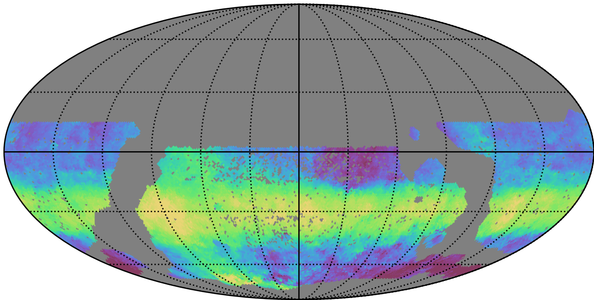
smc_lmc_v3.3_10yrs WFD z band: Median HA
