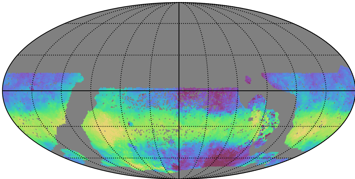
smc_lmc_v3.3_10yrs WFD y band: Median HA
