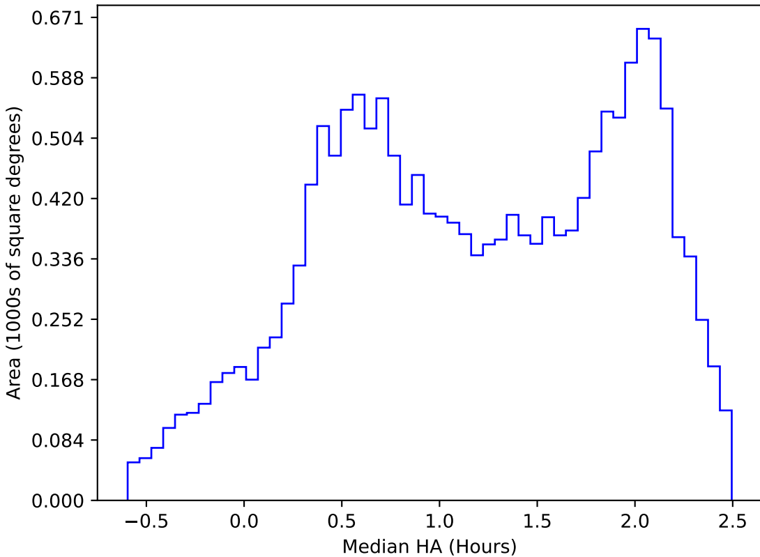
smc_lmc_v3.3_10yrs WFD y band: Median HA
