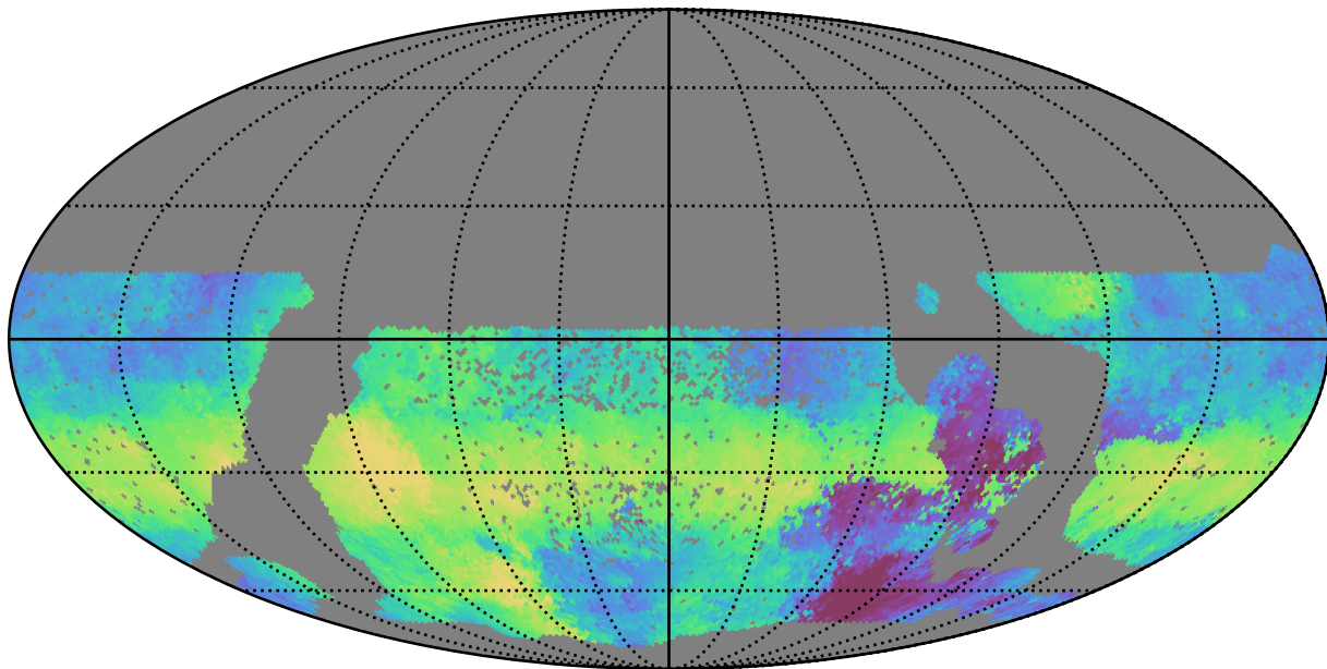
smc_lmc_v3.3_10yrs WFD u band: Median HA
