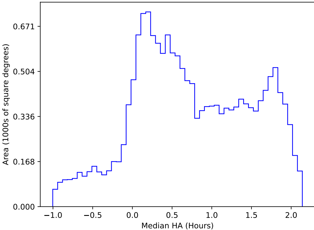
smc_lmc_v3.3_10yrs WFD r band: Median HA
