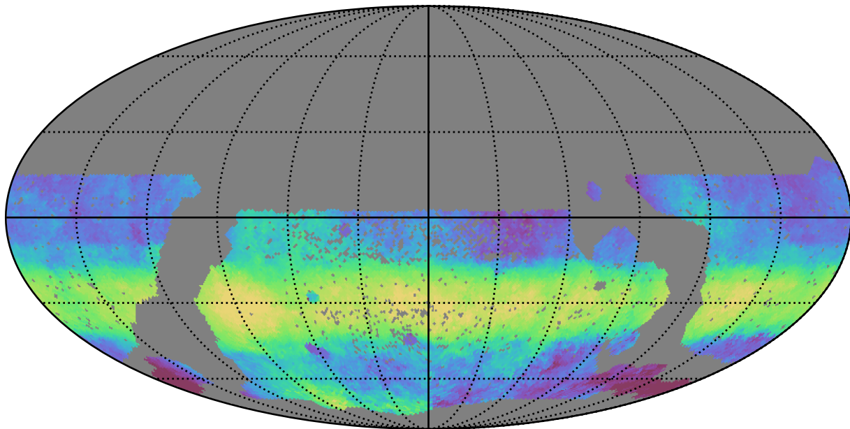
smc_lmc_v3.3_10yrs WFD i band: Median HA
