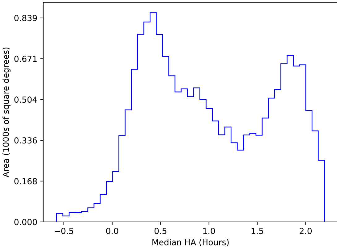
smc_lmc_v3.3_10yrs WFD i band: Median HA
