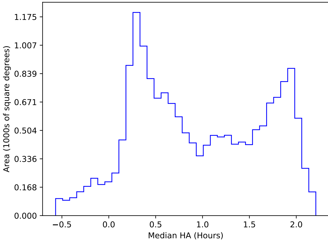
smc_lmc_v3.3_10yrs WFD all bands: Median HA
