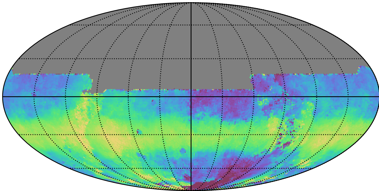
smc_lmc_v3.3_10yrs All sky y band: Median HA
