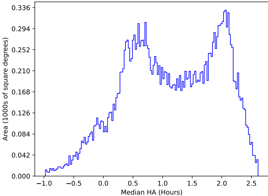
smc_lmc_v3.3_10yrs All sky y band: Median HA
