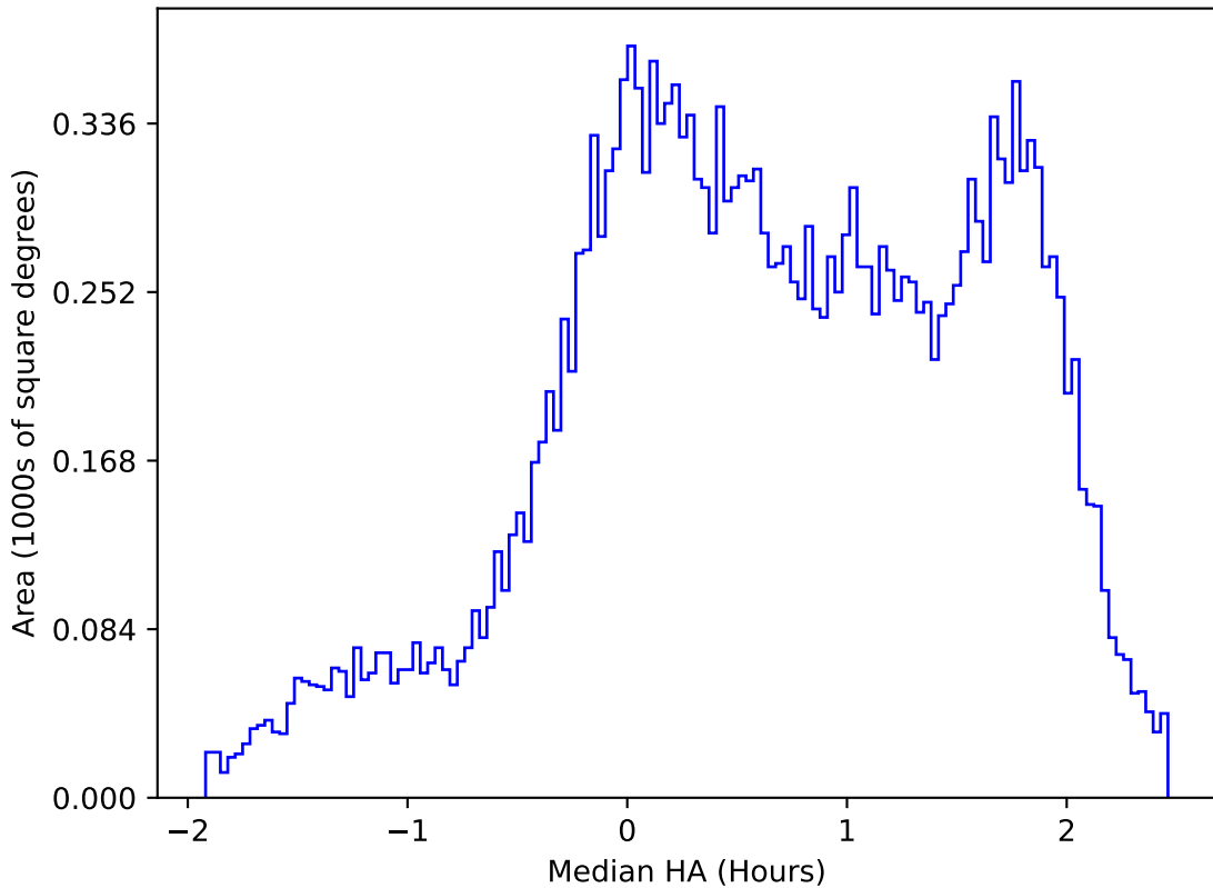
smc_lmc_v3.3_10yrs All sky u band: Median HA
