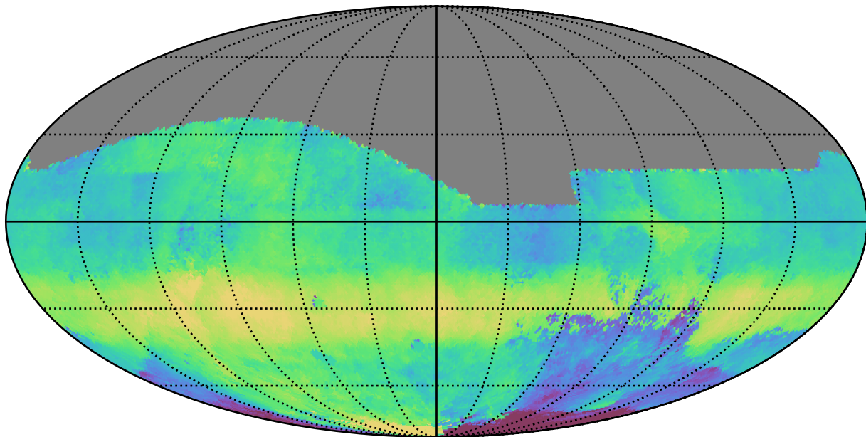
smc_lmc_v3.3_10yrs All sky r band: Median HA
