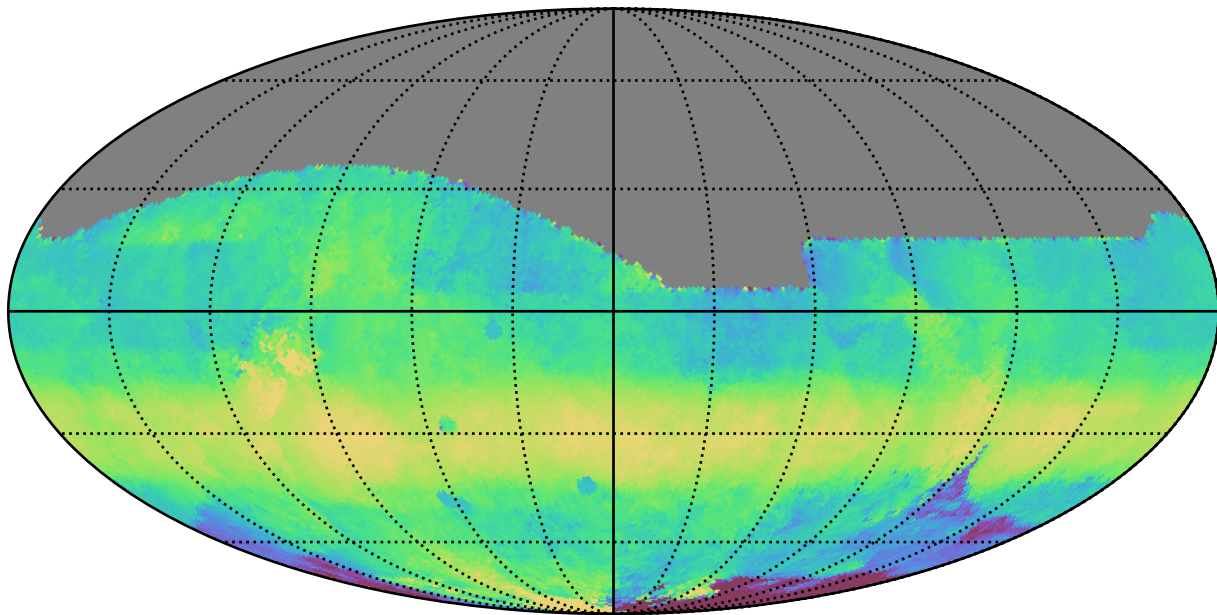
smc_lmc_v3.3_10yrs All sky i band: Median HA
