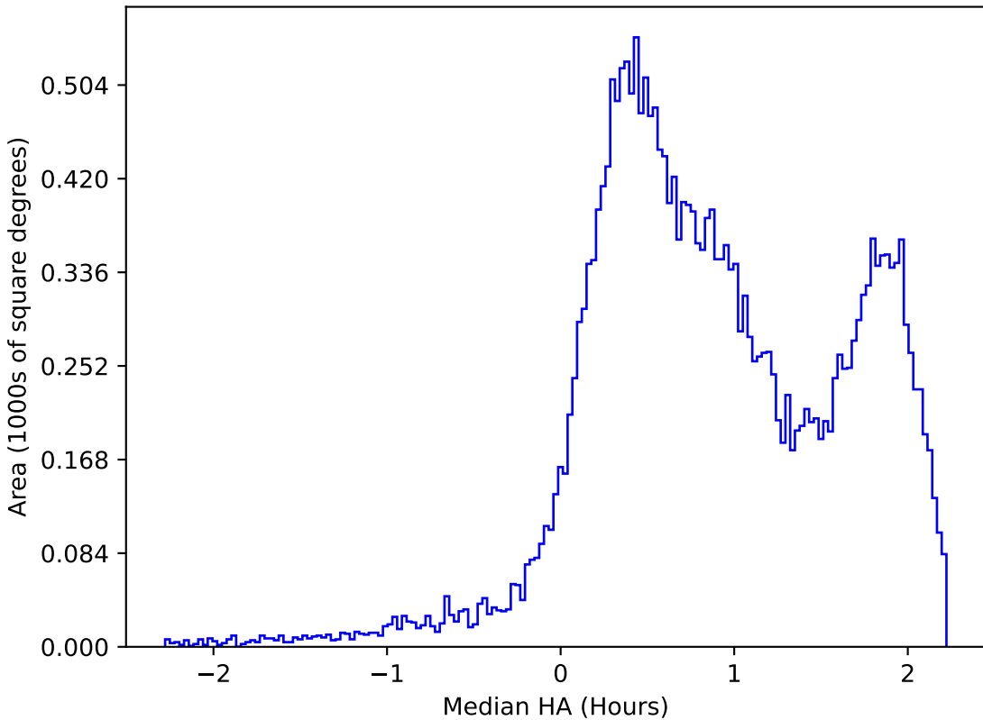
smc_lmc_v3.3_10yrs All sky i band: Median HA
