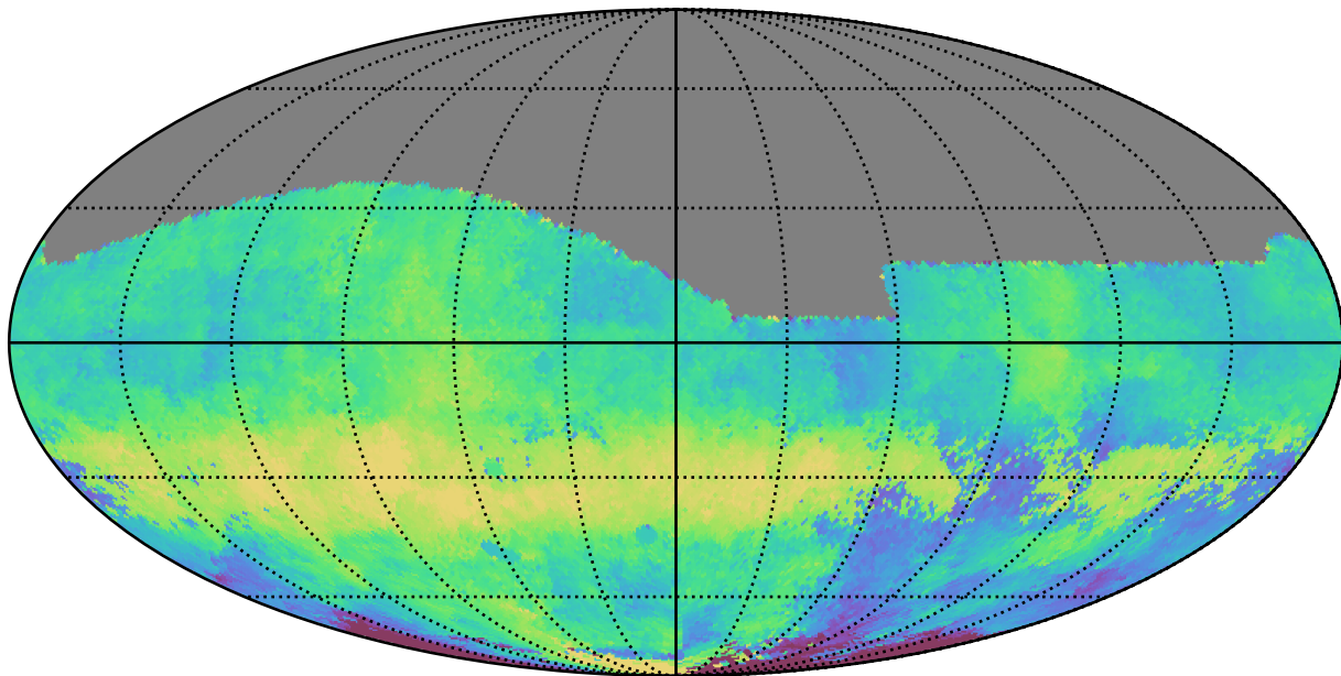
smc_lmc_v3.3_10yrs All sky g band: Median HA
