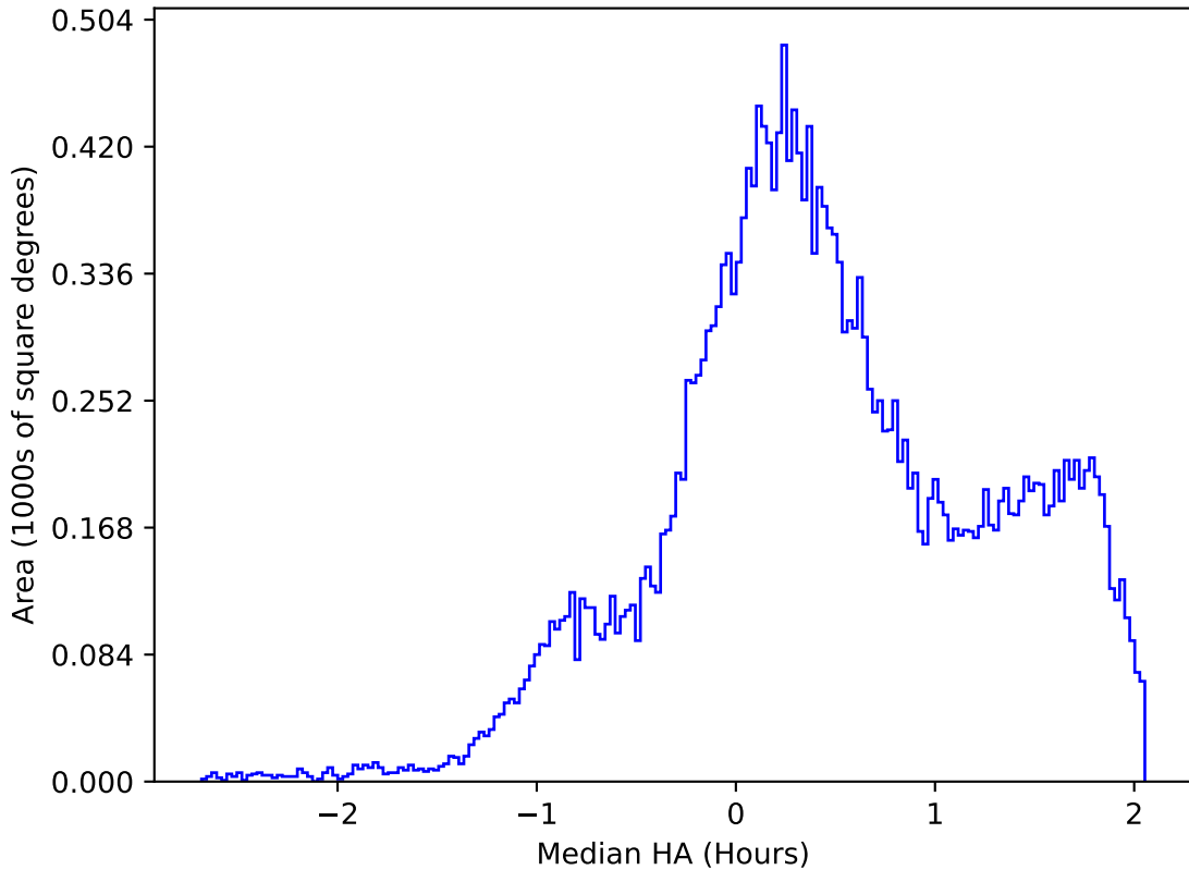
smc_lmc_v3.3_10yrs All sky g band: Median HA
