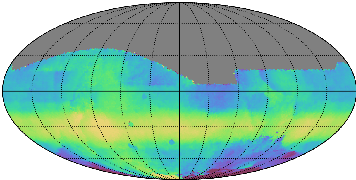
smc_lmc_v3.3_10yrs All sky all bands: Median HA
