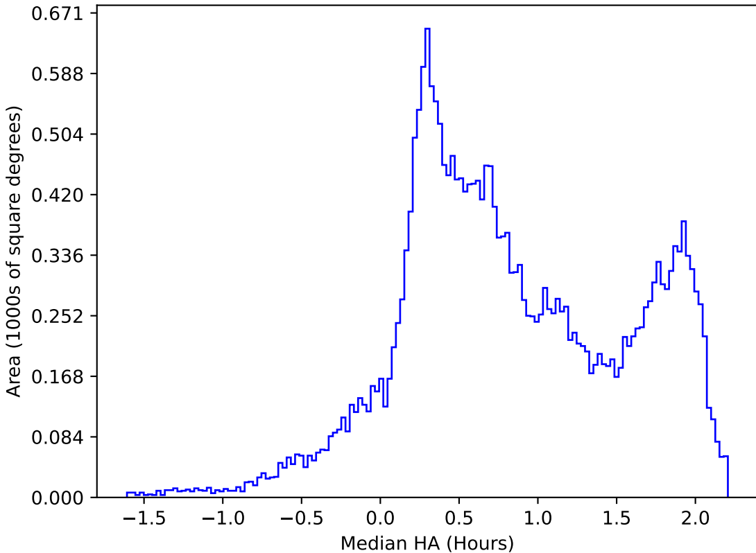
smc_lmc_v3.3_10yrs All sky all bands: Median HA
