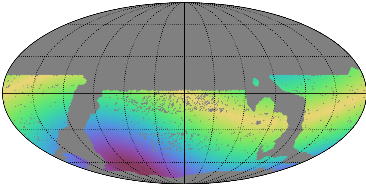
smc_lmc_v3.3_10yrs WFD z band: Max solarElong
