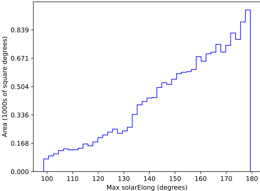
smc_lmc_v3.3_10yrs WFD z band: Max solarElong
