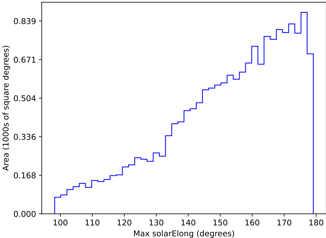
smc_lmc_v3.3_10yrs WFD u band: Max solarElong
