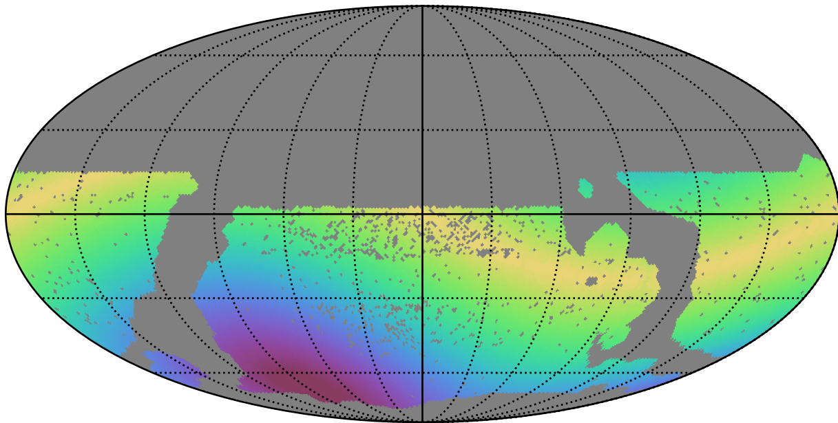
smc_lmc_v3.3_10yrs WFD r band: Max solarElong
