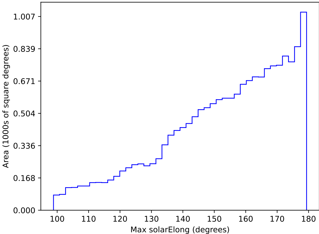
smc_lmc_v3.3_10yrs WFD r band: Max solarElong
