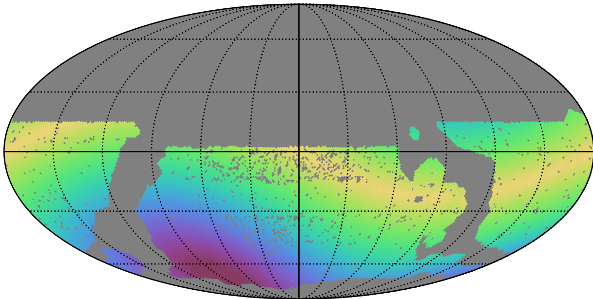
smc_lmc_v3.3_10yrs WFD i band: Max solarElong
