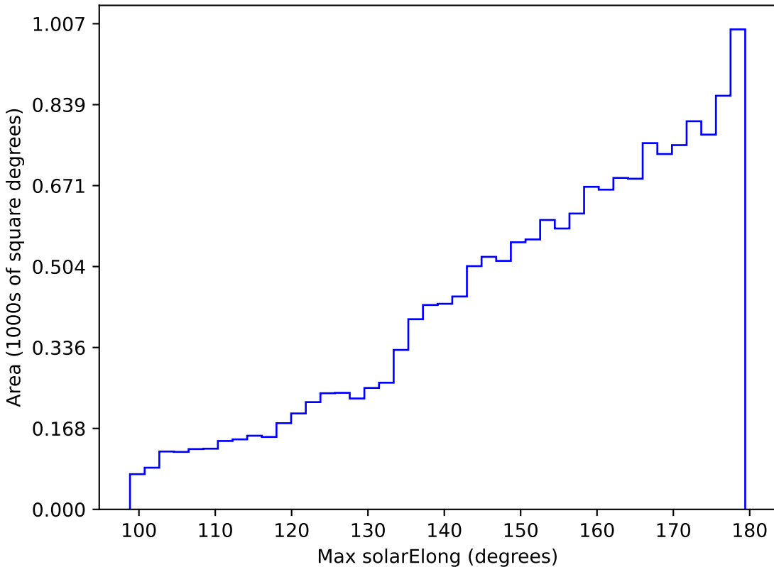
smc_lmc_v3.3_10yrs WFD i band: Max solarElong
